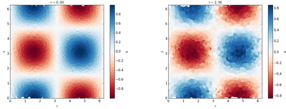
Figure 6: Example snapshots at t = 0 and t = 2.96 showing the deformation of the Voronoi CVs with N_{CV} = 2500 . Contour colored with u velocity.
