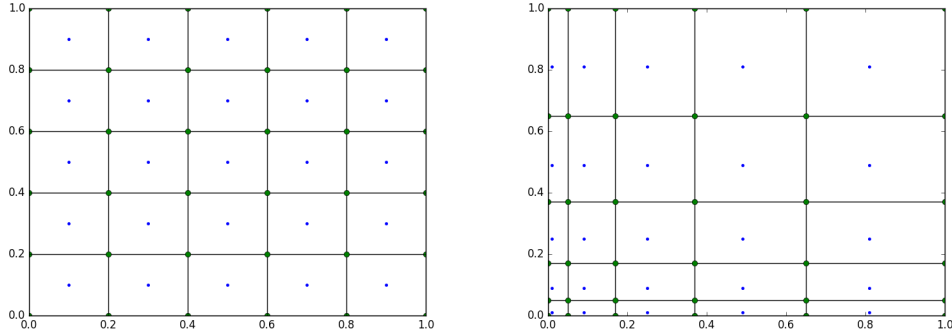
Figure 4: Cartesian grid and stretched grid generated using the scipy.spatial.voronoi library.
