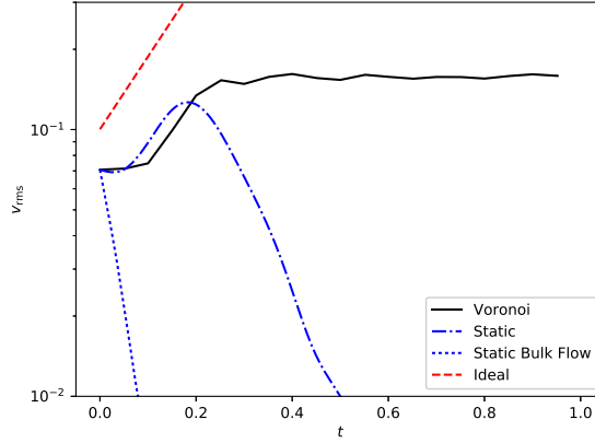
Figure 15: Vertical velocity amplitude growth using N_{CV} = 50^2 cells, showing agreement with the ideal Kelvin-Helmholtz growth rate. This is juxtaposed with the evolution using a static Cartesian grid, which in extreme cases produces an artificially stable solution.
