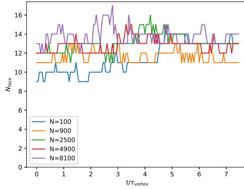
Figure 10: The evolution of the maximum number of faces a single cell contains as the simulation progresses, and for different resolutions.
