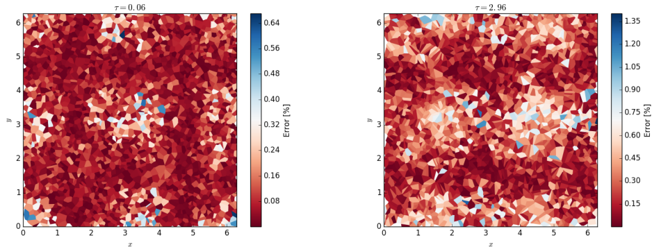
Figure 7: Example snapshots at t = 0.06 and t = 2.96 showing the error contributions per CV in the domain with N_{CV} = 2500 . The error is represented as a percentage error in the given CV with respect to the overall area in the domain, such that each CV is colored with their contributions to the total error in order to display regions where the local error is pronounced.
