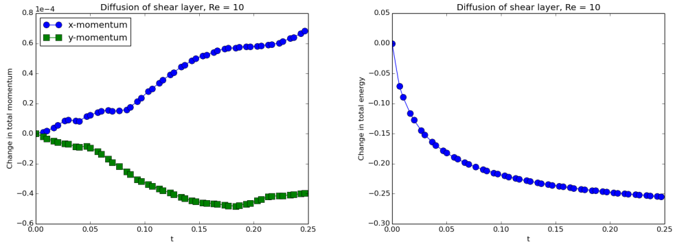
Figure 12: Evolution of momentum (left) and energy (right) in the computational domain over time.
