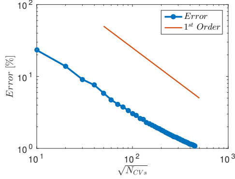
Figure 8: Spatial discretization error computed with Eq. 5 showing first order convergence.
