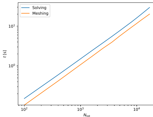
Figure 5: The relative time spent solving and meshing in simulating the Taylor-Green vortex problem for increasing problem size.
