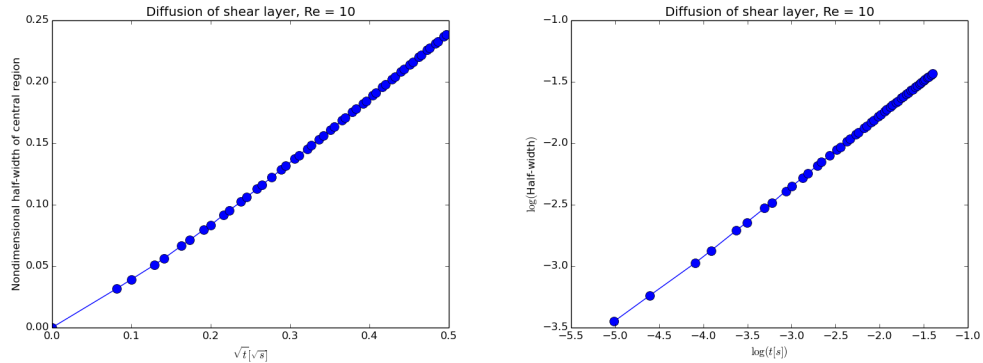
Figure 13: Evolution of the width of the shear layer over time in linear (left) and logarithmic (right) axes.
