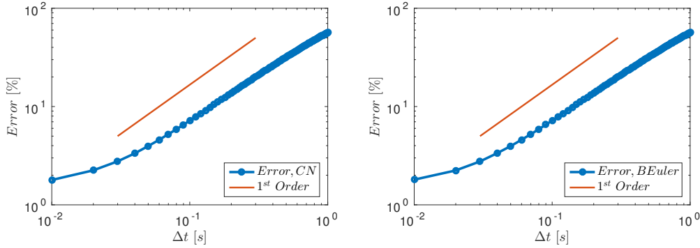
Figure 9: Solver temporal error computed with Eq. 5 showing first order convergence above a threshold \Delta t .
