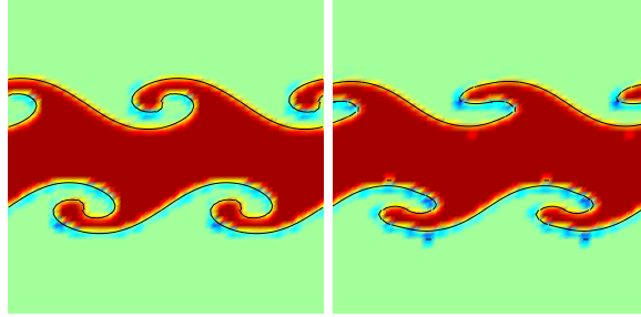
Figure 17: Tracer concentration showing the evolution of the Kelvin-Helmholtz instability for \text{Re} = 10^3 of an initial discontinuous shear band, shown at \tau = 0.85 e -folding times for N = 64^2 on a uniform cartesian grid without a bulk translational velocity u_b = 0 (left) and with translational bulk velocity u_b = 100 (right).
