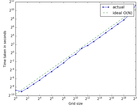
Figure 3: Complexity of meshing process estimated to be O(N) up to 1 million grid cells.
