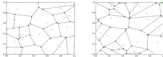
Figure 2: Illustration of bounded domain and periodic domain created by mirroring and repeating the sites outside the domain of interest.
