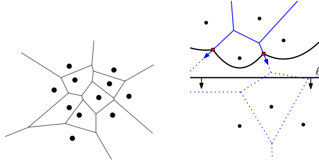
Figure 1: Schematic of a Voronoi diagram and its construction using the line sweep algorithm . The solid black curves on the right figure represent the beach line , the horizontal line represents the sweep line and the red squares represent the break points .
