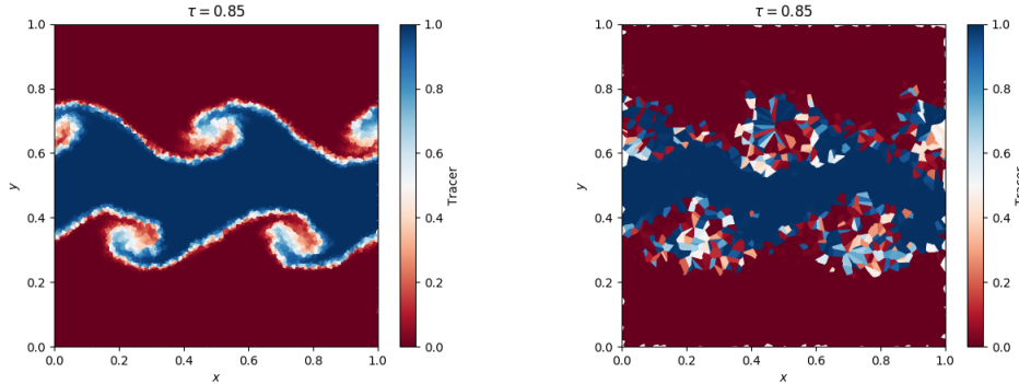
Figure 14: Tracer concentration showing the evolution of the Kelvin-Helmholtz instability for \text{Re} = 10^3 of an initial discontinuous shear band, shown at t = 0.85 e -folding times for N_{CV} = 150^2 cells (left) and N_{CV} = 50^2 cells (right).
